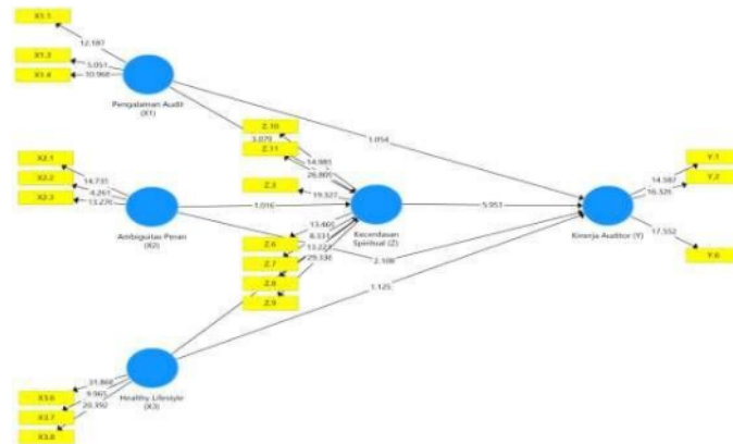
Gambar 1 : Skema Outer Model
