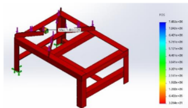
Gambar 10. Simulasi Faktor Keamanan ( Factor of Safety )
