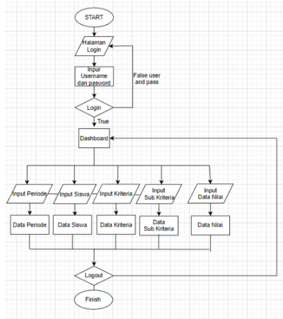
Gambar 3.1 Flowchart Admin
