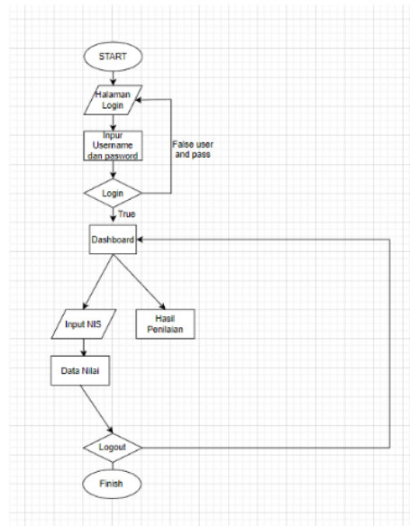
Gambar 3.2 Flowchart User
