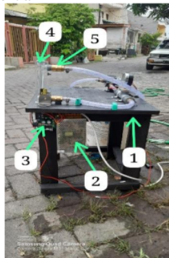
Gambar 3. Instalasi Penelitian 1
