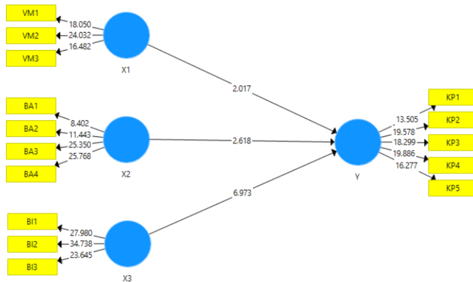
Gambar 1. Bootstrapping Test Result
