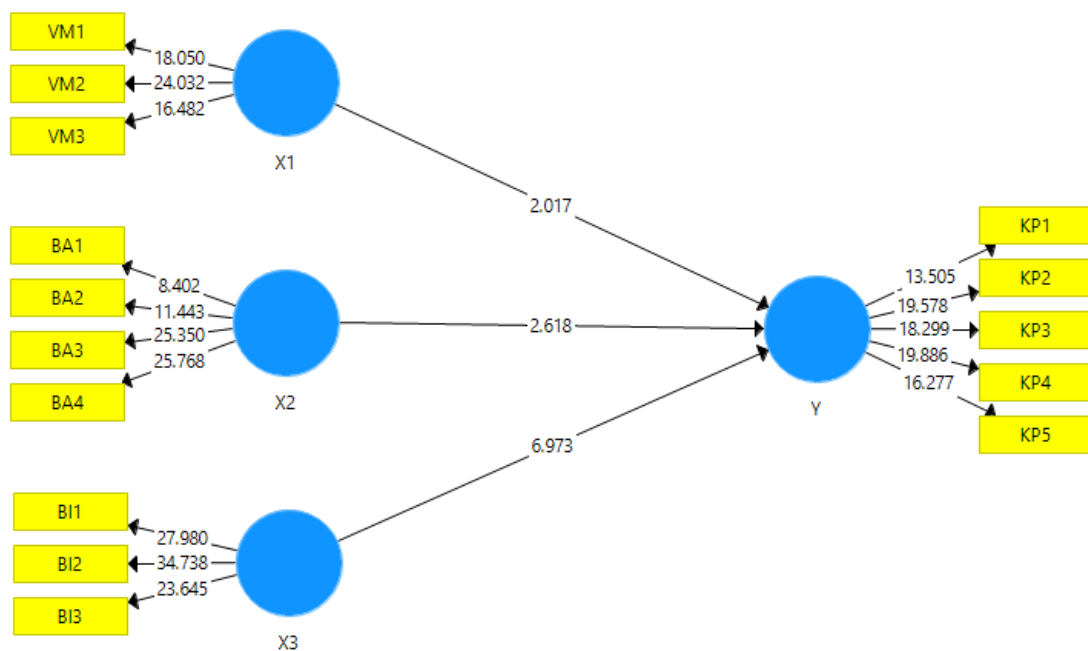
Gambar 1. Bootstrapping Test Result
