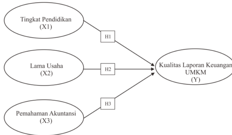
Gambar 1: Kerangka Penelitian
