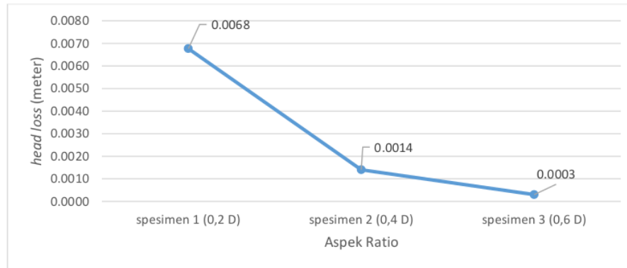
Gambar 10. Head Loss Sudden Contraction
