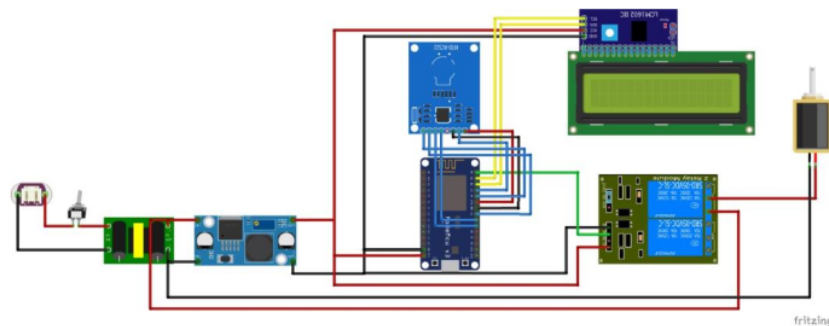
Gambar 3. Wiring Diagram
