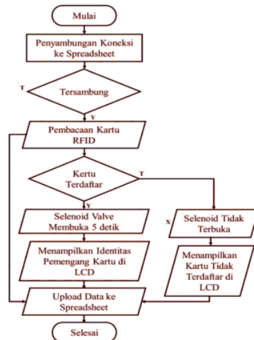
Gambar 2. Flowchart
