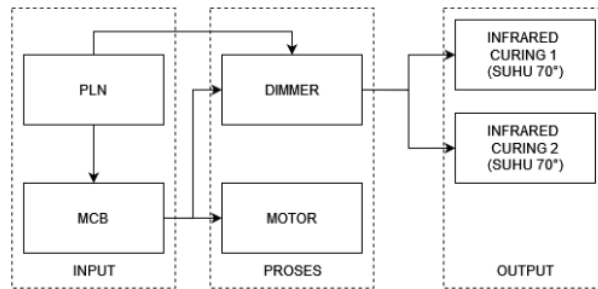
Gambar 1. Blok Diagram
