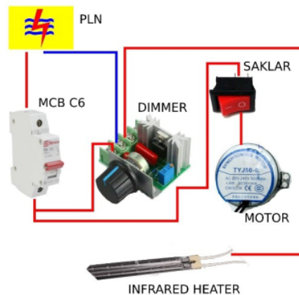
Gambar 2. Wiring Diagram
