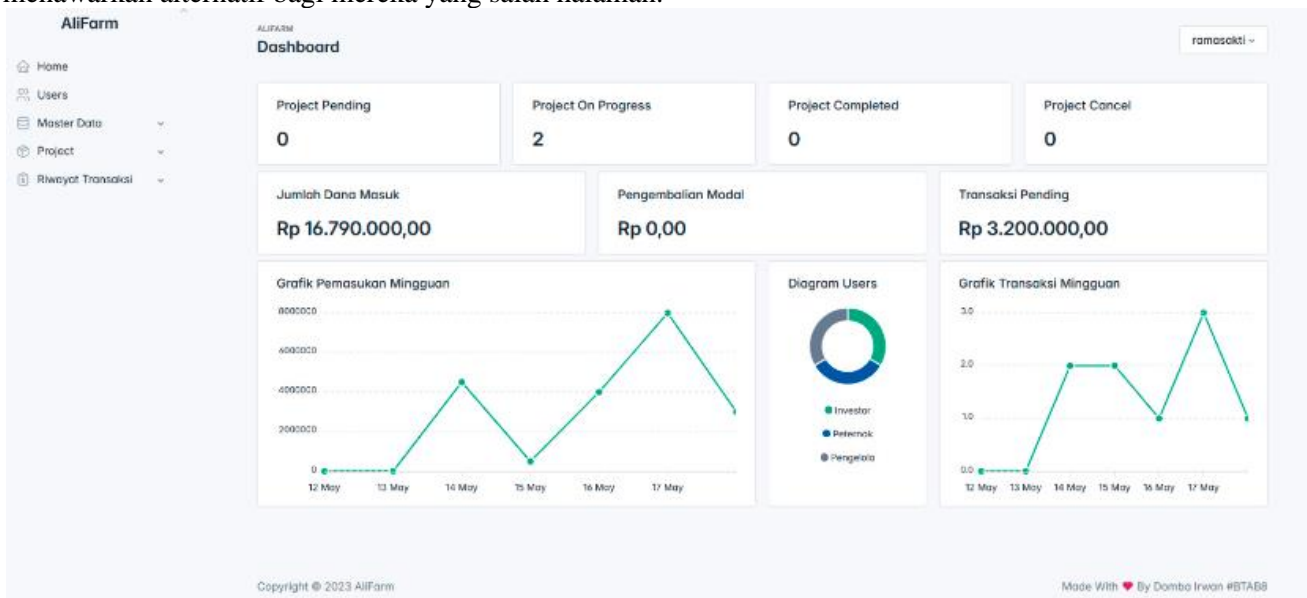
Gambar 15. Tampilan Dashboard
