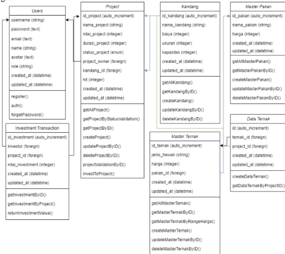
Gambar 10. Class Diagram
