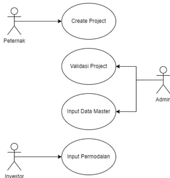
Gambar 5. Usecase Diagram
