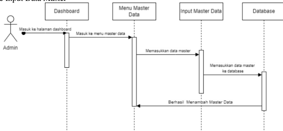
Gambar 8. Squence Input Data Master
