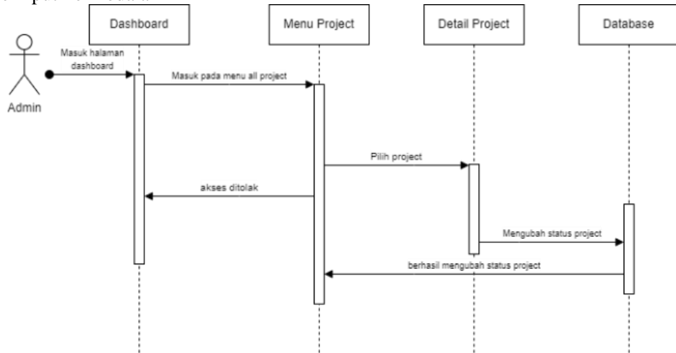
Gambar 9. Sequence Input Permodalan
