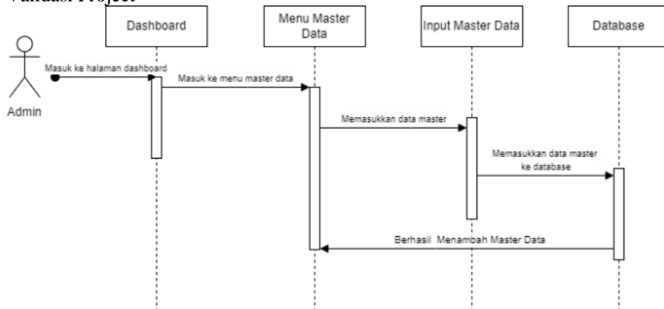
Gambar 7. Squence Validasi Project
