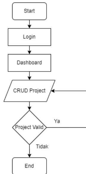
Gambar 4. Flowchart Peternak
