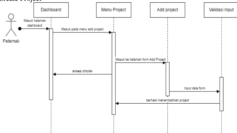
Gambar 6. Squence Create Project
