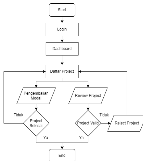
Gambar 3. Flowchart Admin
