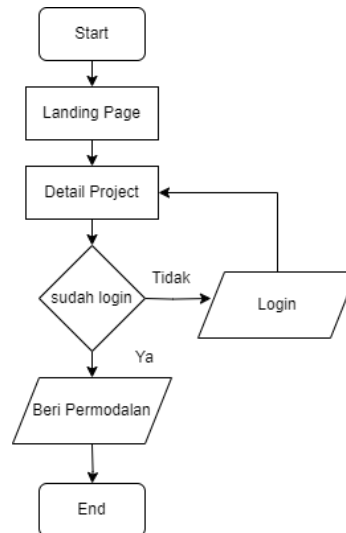
Gambar 2. Flowchart Investor
