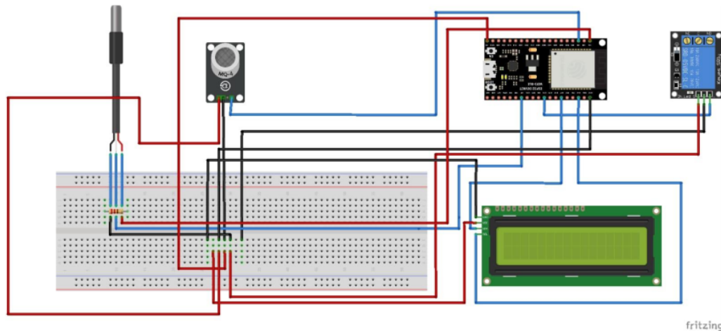
Gambar 3. Wiring Diagram
