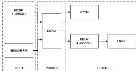
Gambar 1. Blok Diagram
