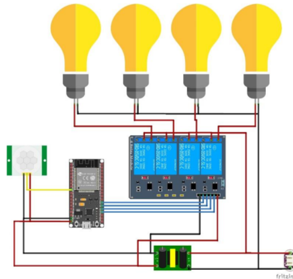
Gambar 3. Wiring Diagram
