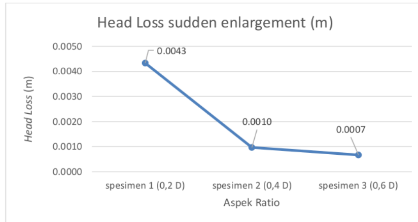
Gambar 6. Head Loss Sudden enlargement
