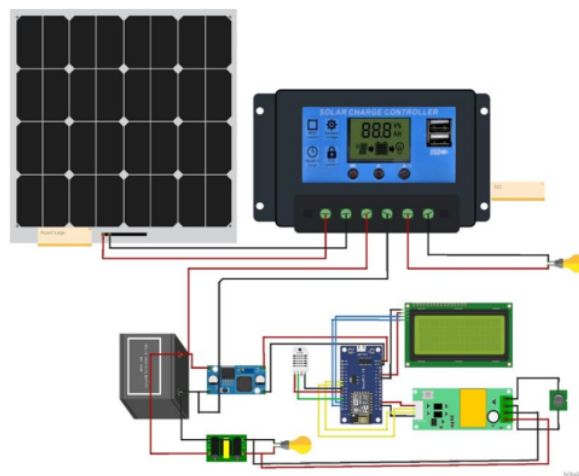
Gambar 3. Wiring Diagram
