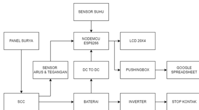
Gambar 1. Blok Diagram
