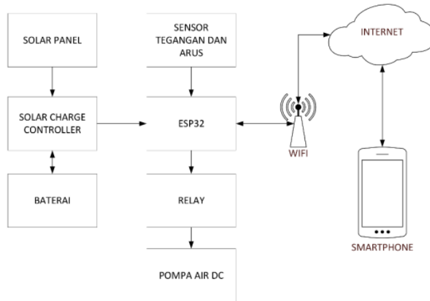
Gambar 1. Blok Diagram
