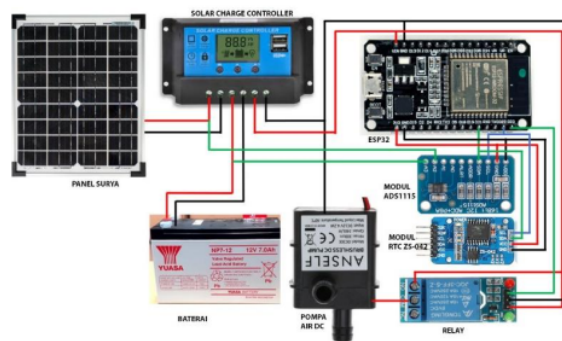
Gambar 2. Wiring Diagram
