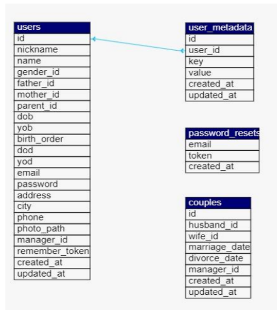
Gambar 6. ERD (Entity Relationship Diagram)
