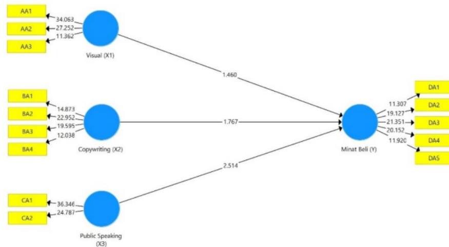
Gambar 4.1 Bootstrapping Test Result
