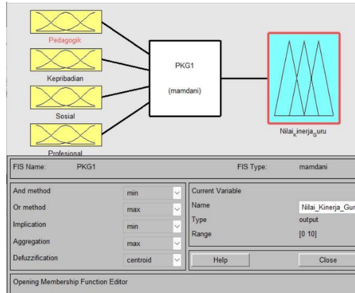
Gambar 5. Model logika fuzzy mamdani
