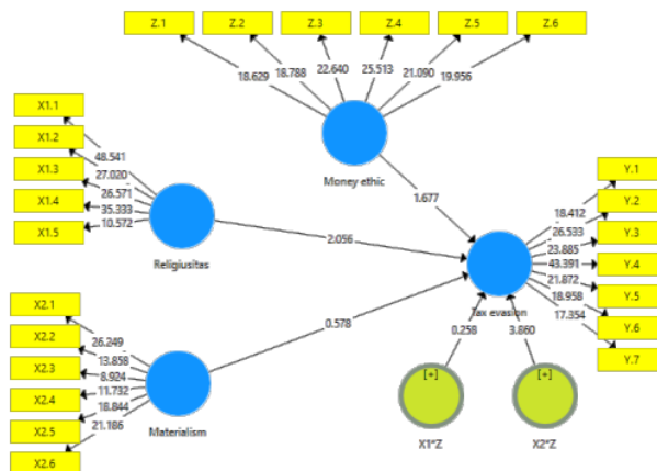
Gambar 3. Hasil Bootstrapping
