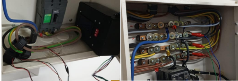
18 Gambar 4. Proses Pengujian Sensor PZEM-004T
