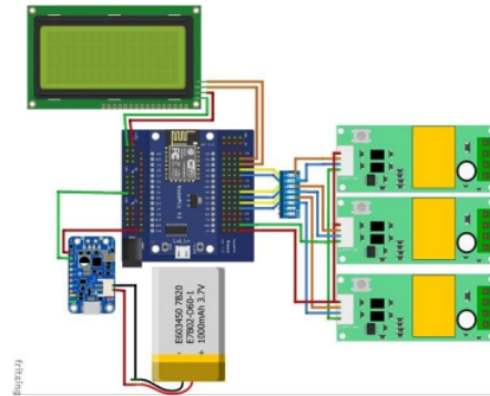
Gambar 3. Wiring Diagram
