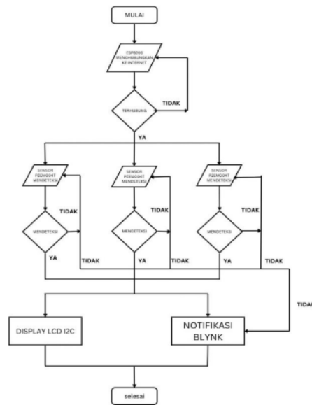
Gambar 2. Flowchart
