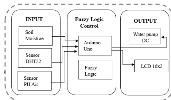
Gambar 1. Blok Diagram
