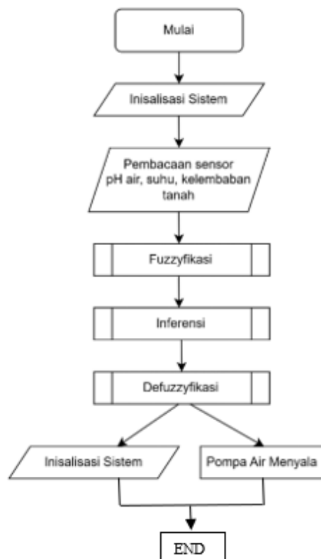
Gambar 2. Flowchart
