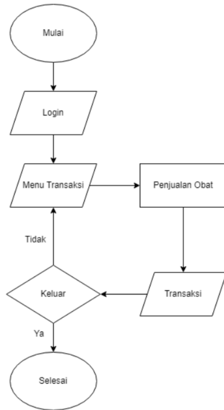
Gambar 3. Flowchart User
