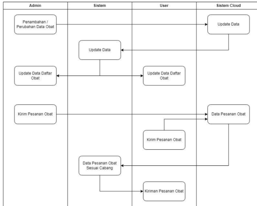
Gambar 6. Sequence Diagram Sistem Informasi Apotek
