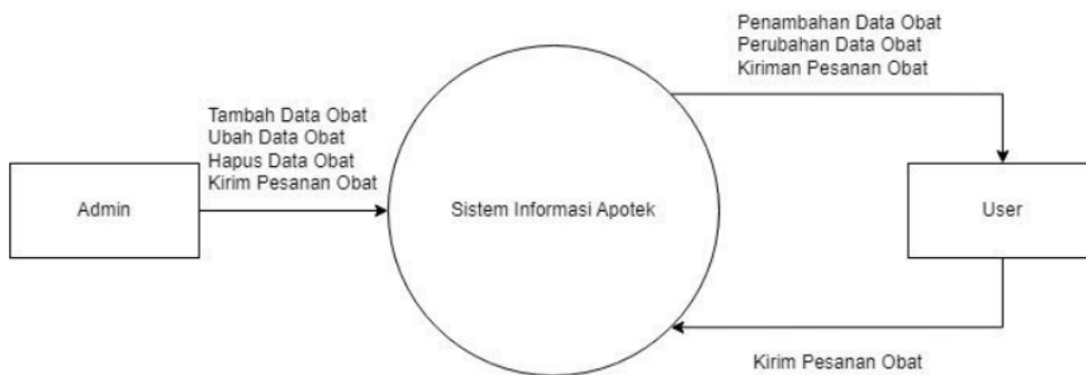
Gambar 4. DFD Level 0
