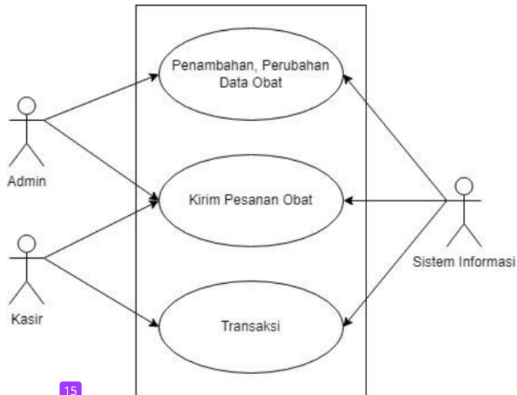
15 Gambar 6. Use Case Diagram Sistem Informasi Apotek
