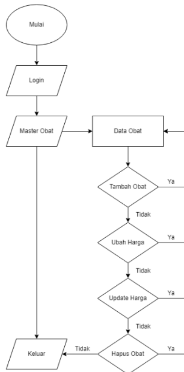
Gambar 2. Flowchart Admin
