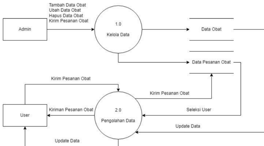
Gambar 5. DFD Level 1
