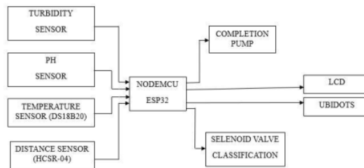
Gambar 1. Block Diagram
