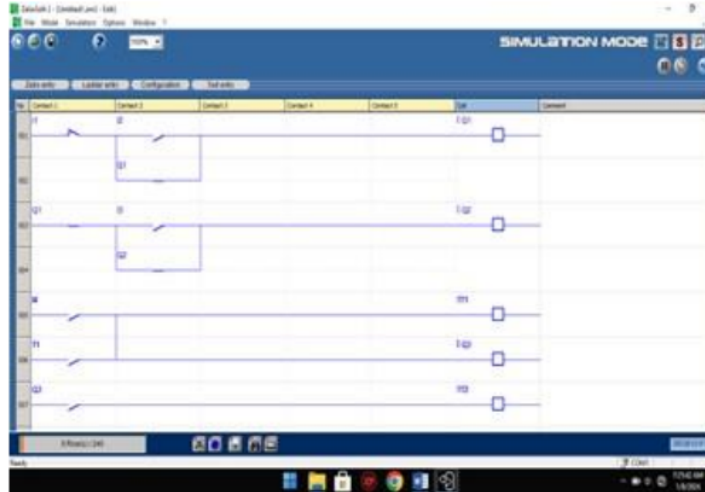
Gambar 5. Program Ladder Diagram Smart Relay
