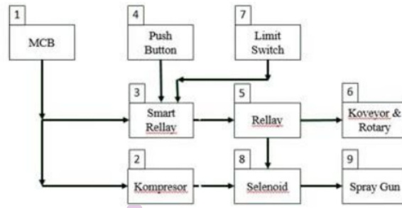
Gambar 2. Blok Diagram
