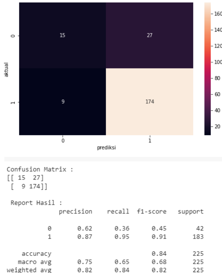
Gambar 9. Hasil Confusion Matriks
