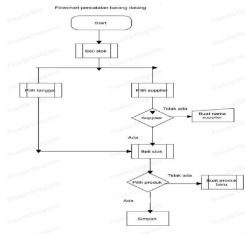
Gambar 1 Flowchart barang masuk
