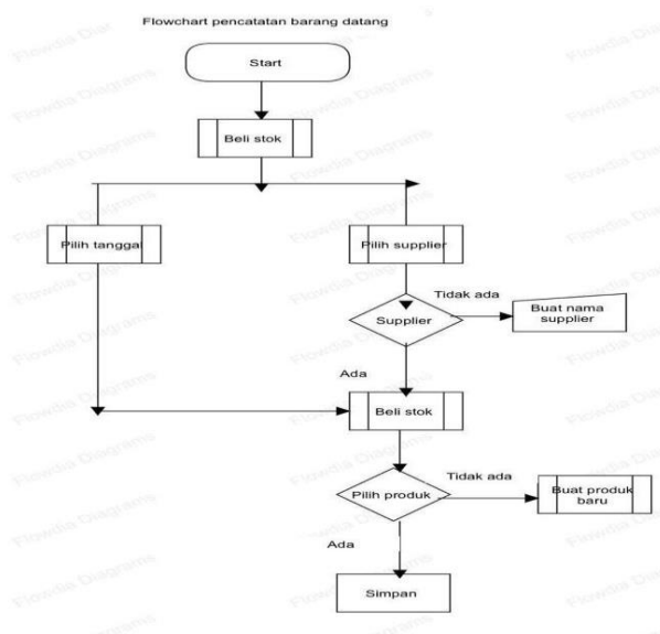
Gambar 1 Flowchart barang masuk
