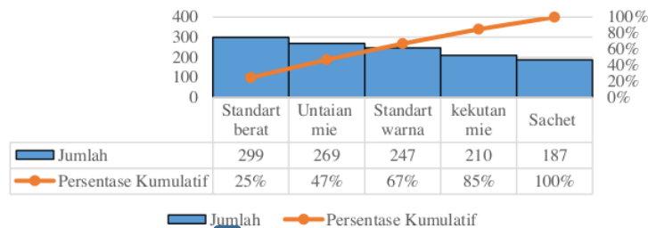
Gambar 2. Diagram pareto
