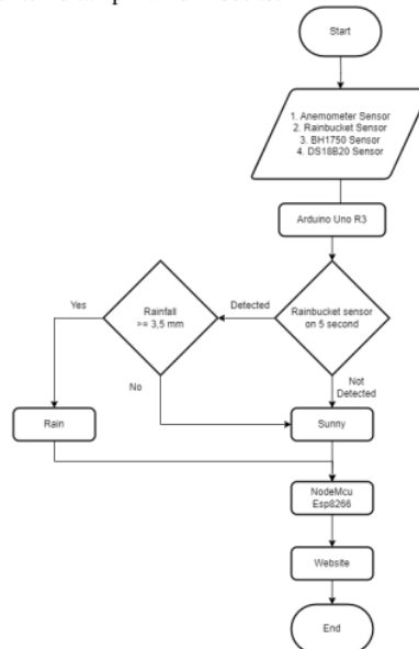
Gambar 2. Flow Diagram
