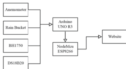
Gambar 1. Blok Diagram
