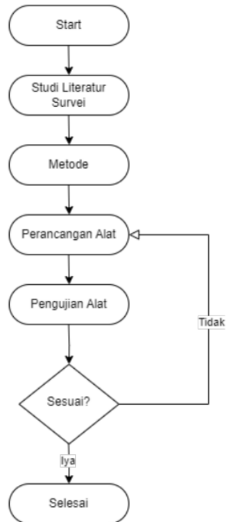
Gambar 1. Flowchart Penelitian
