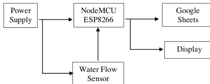
Gambar 2. Blok Diagram System
