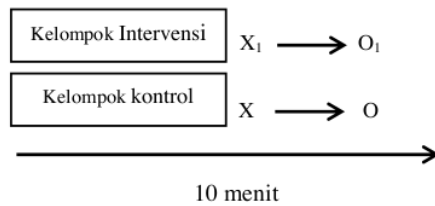
Gambar 1: Desain penelitian
