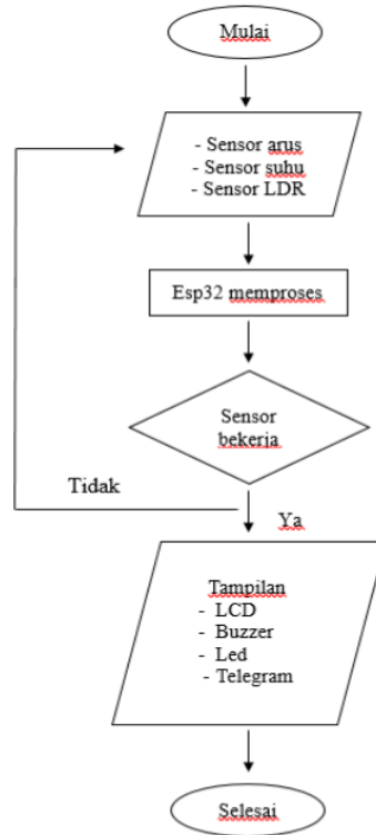
Gambar 3. Flowchart Alat
