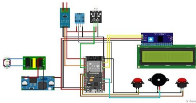
Gambar 1. Wiring Diagram
