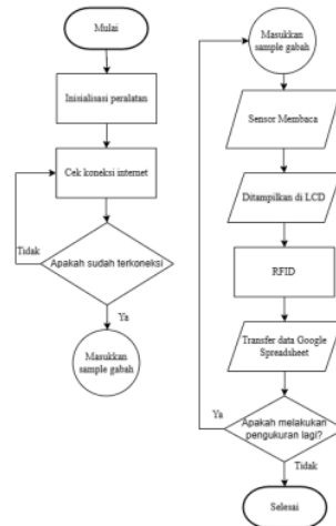
Gambar 2. Diagram Alir
