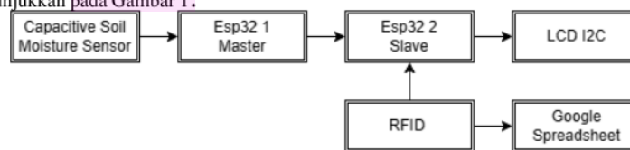
Gambar 1. Blok Diagram
