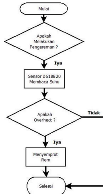
Gambar 3. Diagram alir
