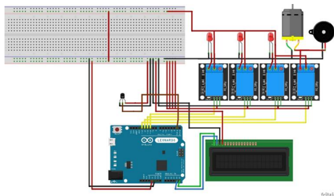
Gambar 1. wiring system
