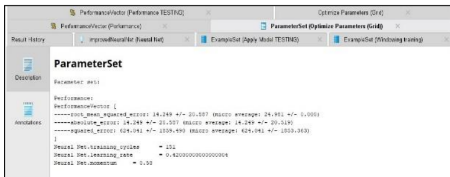
Gambar 2. Hasil RMSE
