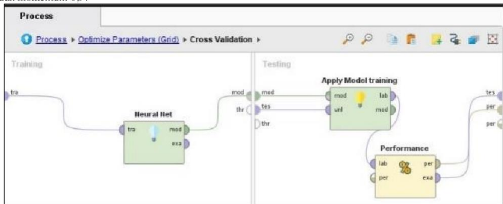
Gambar 4. Subproses Crossvalidation
