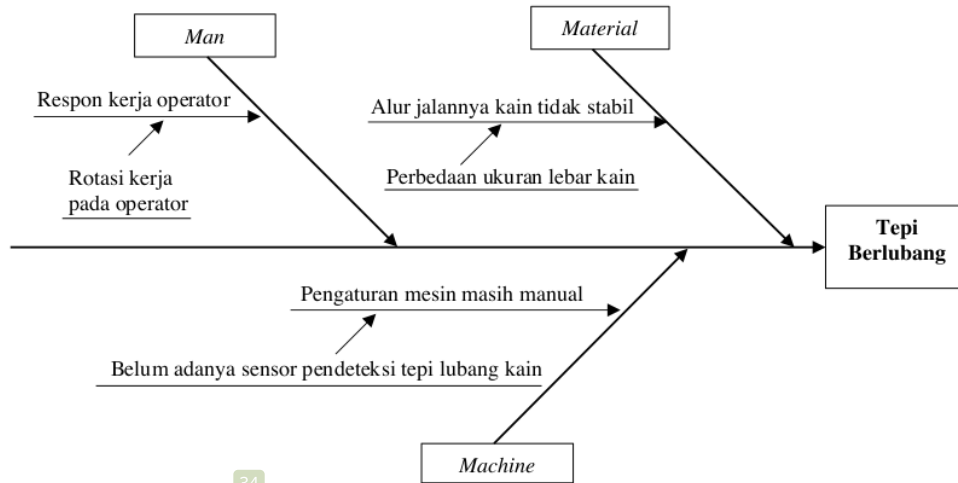
Gambar 5. Diagram Fishbone Cacat Tepi Berlubang
