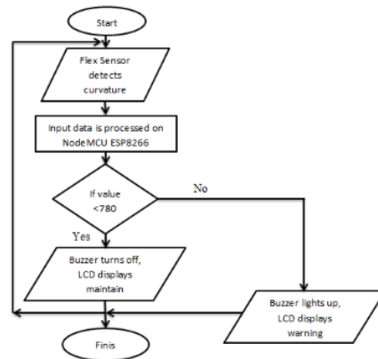
Gambar 2. Diagram Flow Chart
