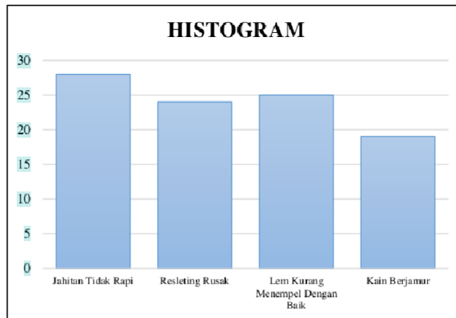
Gambar 3. Histogram
