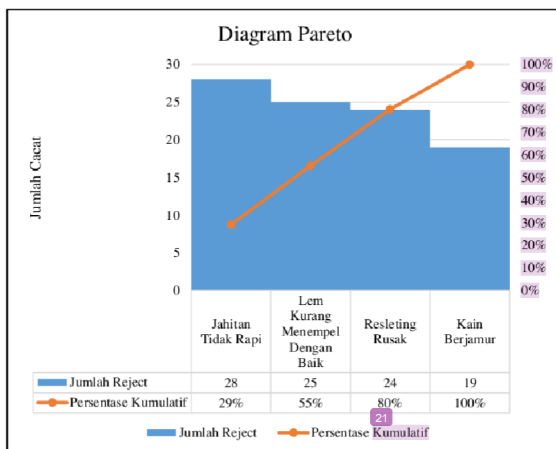
Gambar 4. Diagram Pareto
