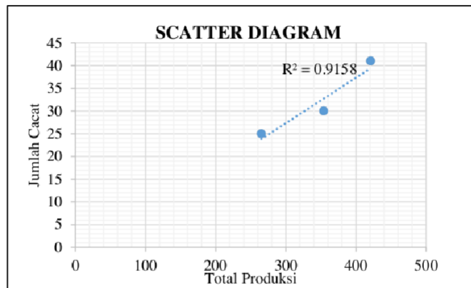
Gambar 5. Scatter Diagram
