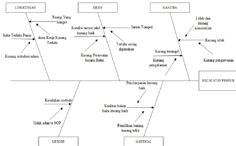
Gambar 7. Fishbone Diagram
