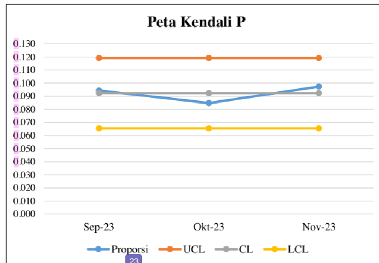
Gambar 6. Peta Kendali
