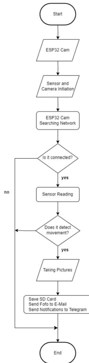
Gambar 4. Flowchart
