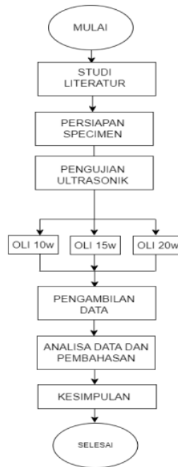
Gambar 8 Flowchart
