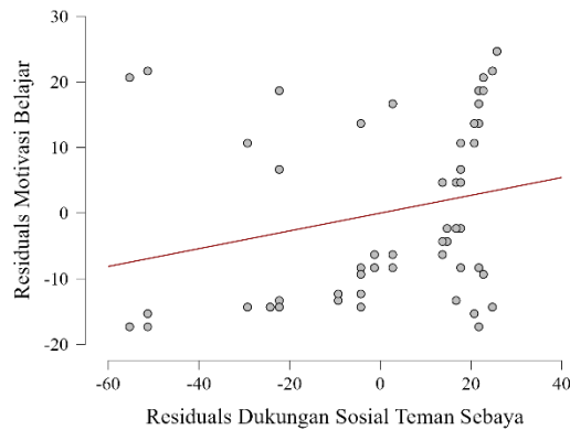
Gambar 1. Scatter Plot data Penelitian
