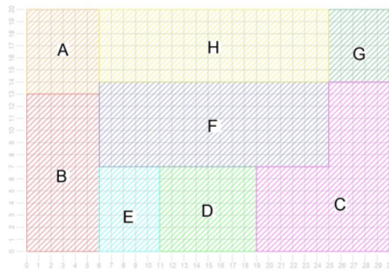
Gambar 6. Layout Usulan 3
