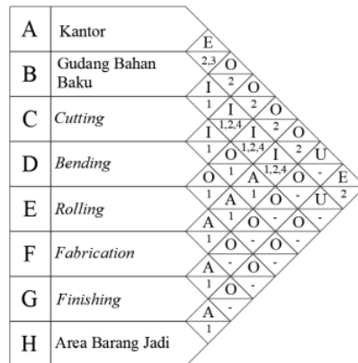
Gambar 3. Activity Relation Chart
