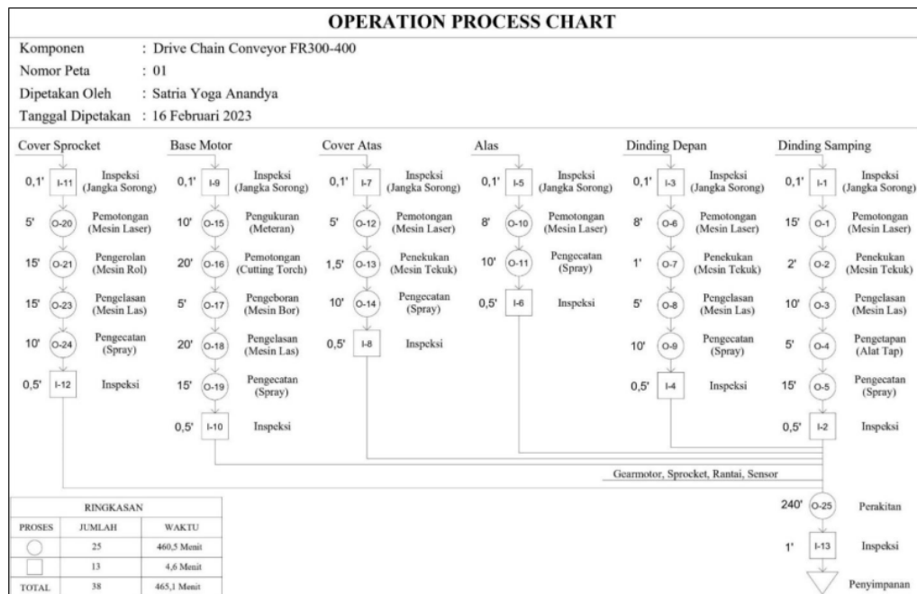
Gambar 2. Operation Process Chart Drive Chain Conveyor
