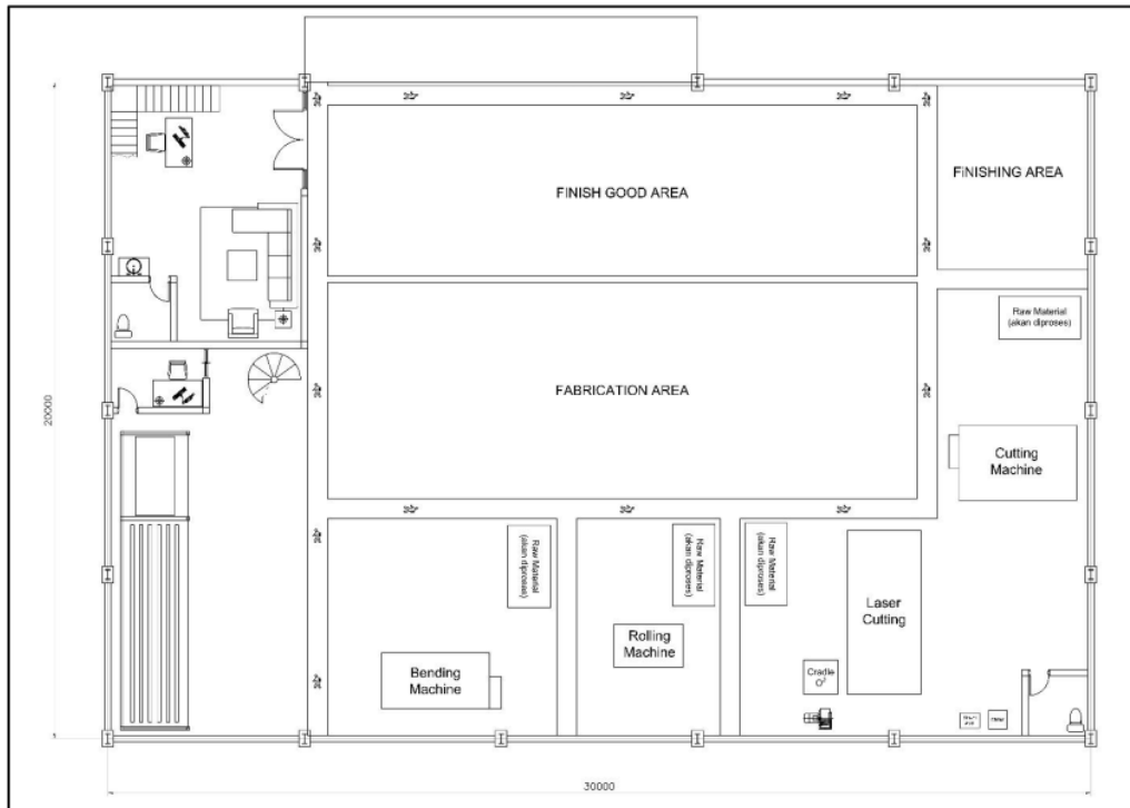
Gambar 7. Layout Usulan 2
