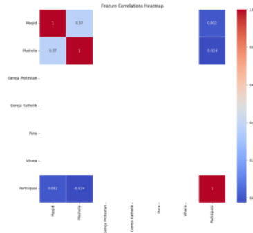
Gambar 7. Correlations Heatmap
