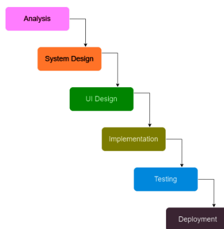
Gambar 1. Metode Waterfall
