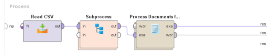
Gambar 3.3 Text Preprocessing
