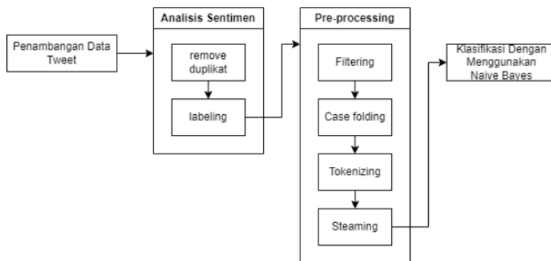
Gambar 1 Diagram Alur Tahapan Penelitian
