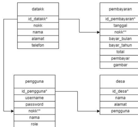
Gambar 5 database
