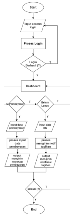
Gambar 2 Flowchart pengurus
