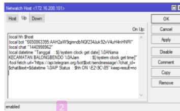
Gambar 3. Script up netwatch mikrotik
