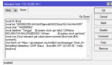
Gambar 4. Script down netwatch mikrotik
