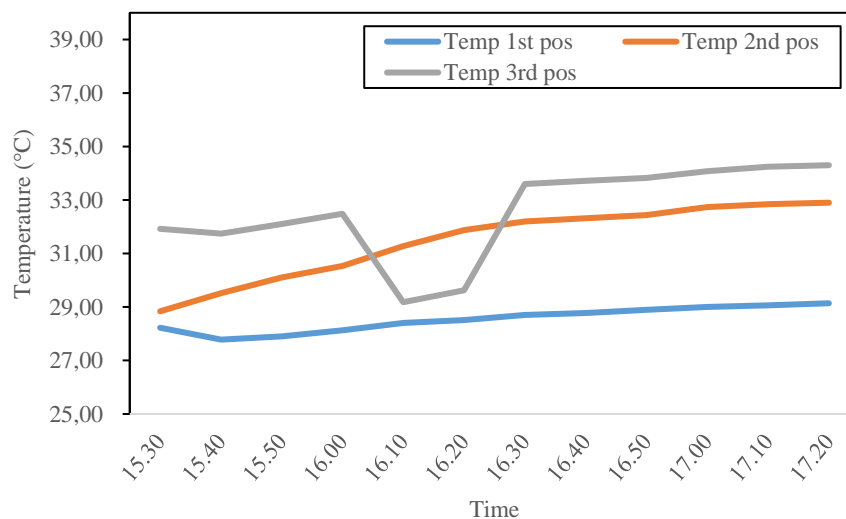
Gambar 11. Temperature Posisi 1,2,3
