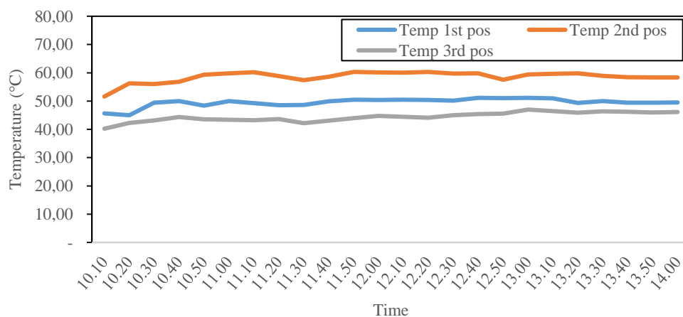
Gambar 7. Temperature Posisi 1,2,3
