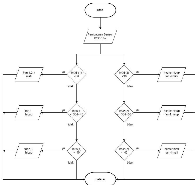
Gambar 4. Diagram Alir
